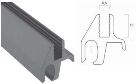
52.3411 Lodret glasholderprofil
